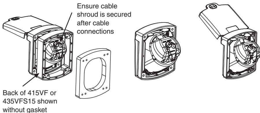
Mounting Flange
