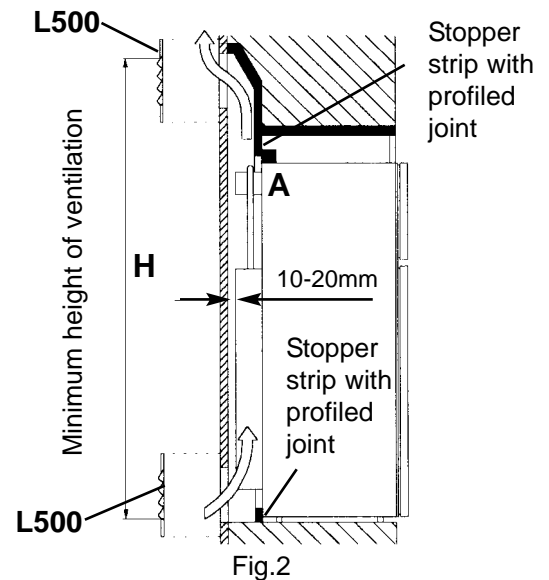
Installation of lower and upper ventilation grilles (L500).
