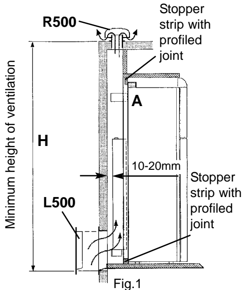
Installation of lower ventilation grille (L500) with roof exhaust (R500).
